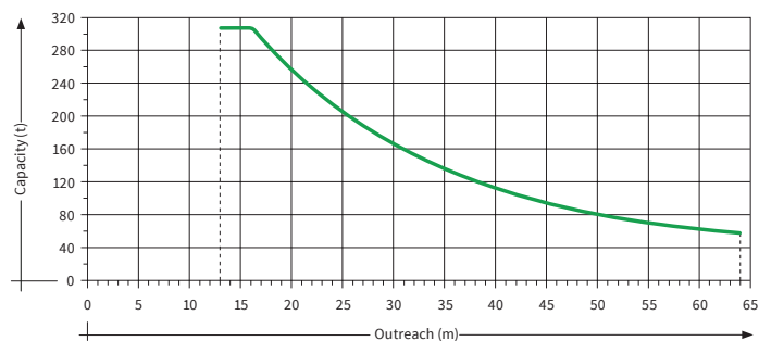
Load Diagram
