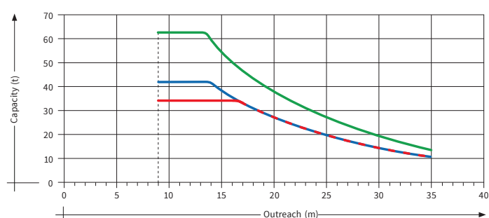
Load Diagram
