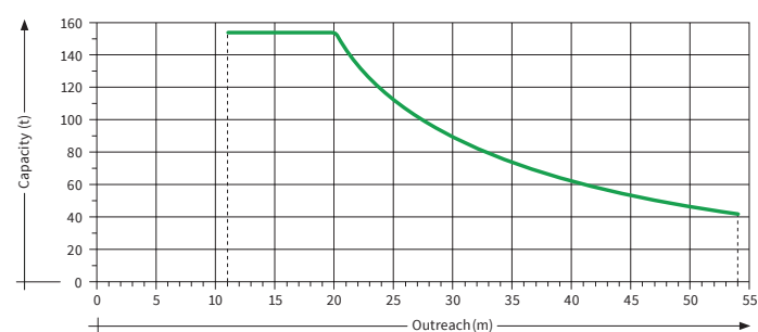
Load Diagram
