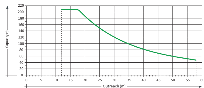
Load diagram
